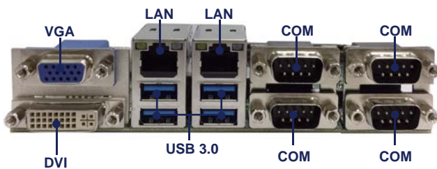
31610 AW/CW Rear I/O
